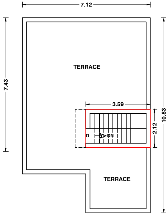
HEAD ROOM PLAN
