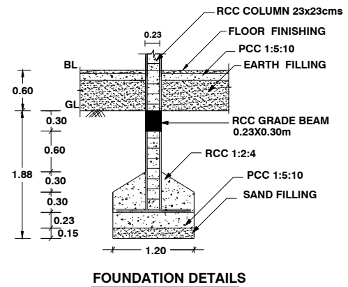
FOUNDATION DETAILS
