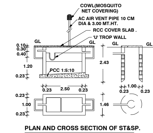
PLAN AND CROSS SECTION OF ST&SP.
