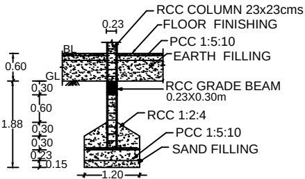
FOUNDATION DETAILS
