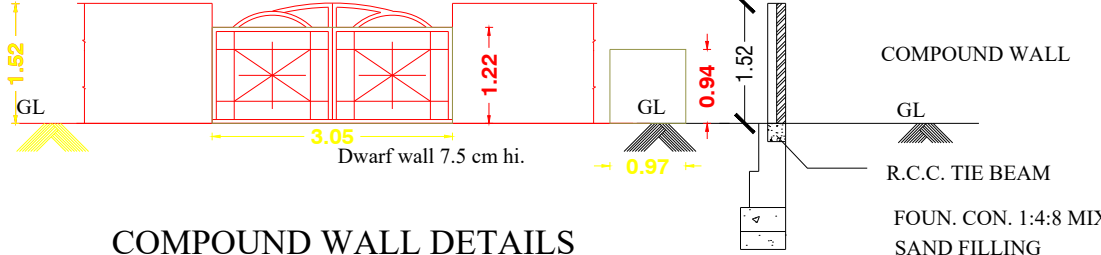
COMPOUND WALL DETAILS
