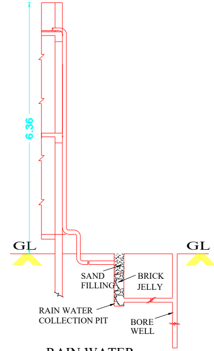
RAIN WATER HARVESTING SYSTEM RWH_CAPACITY_L=1000LTRS
