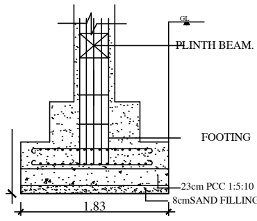
COLUMN FOUNDATION DETAILS NOT TO SCALE
