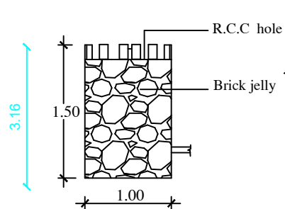
COLLECTING RAIN WATER PIT Not to Scale
