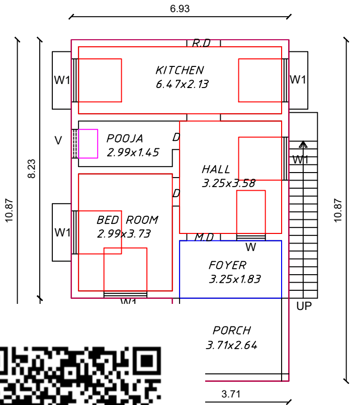
FLOOR PLAN
