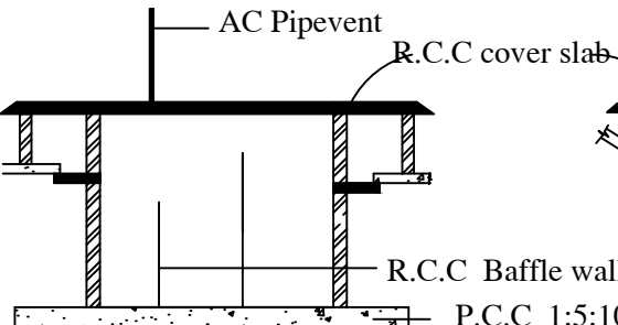
SEPTIC TANK
