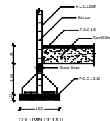
COLUMN DETAIL
