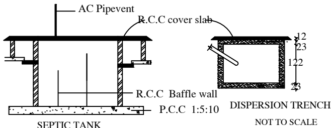
SECTION
