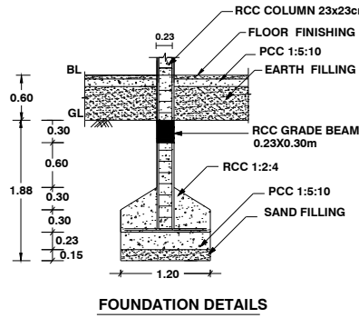
FOUNDATION DETAILS
