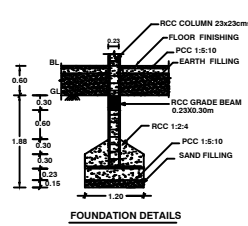
FOUNDATION DETAILS
