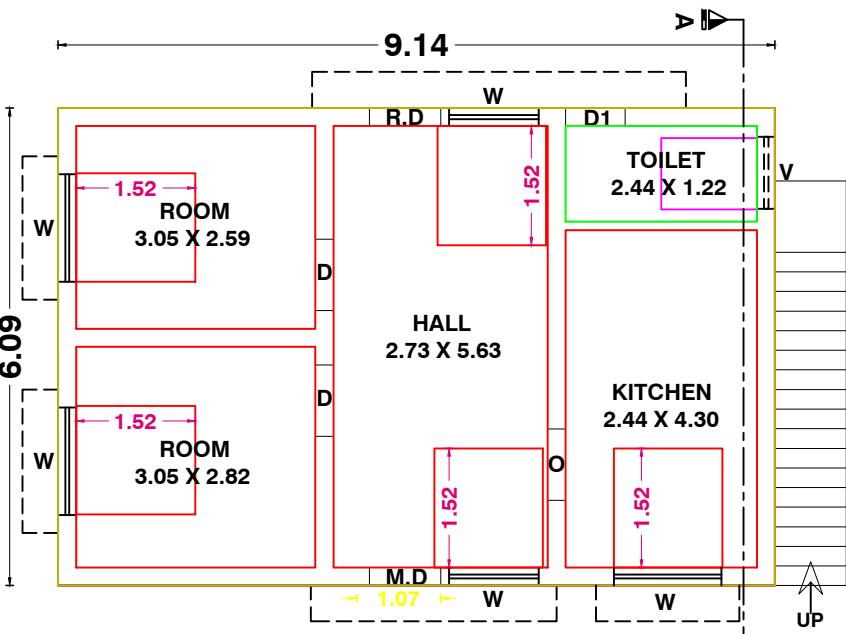
EXI.GROUND FLOOR PLAN
