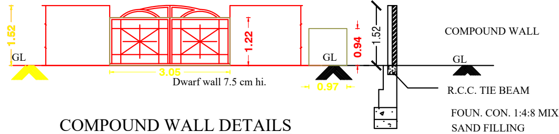
SECTION
