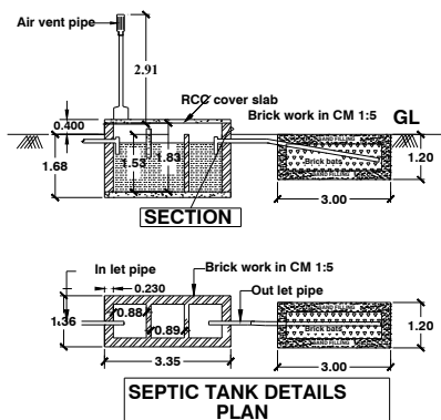
SEPTIC TANK DETAILS PLAN
