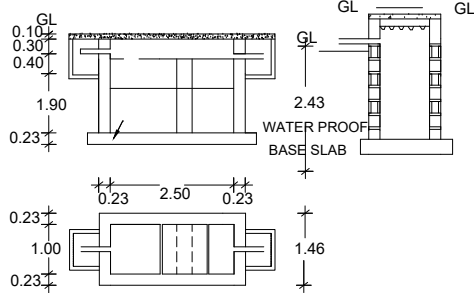
PLAN AND CROSS SECTIONAA & BB OF SEWAGE WASTE TANK
