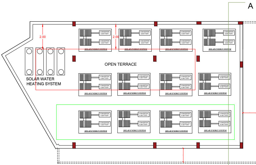
TERRACE PLAN
