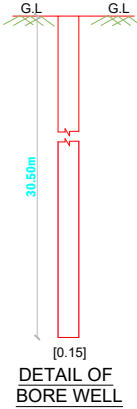
DETAIL OF BORE WELL
