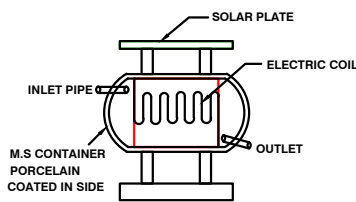
SOLAR SYSTEM
