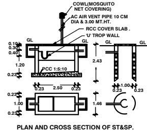
PLAN AND CROSS SECTION OF ST&SP.
