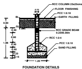
FOUNDATION DETAILS
