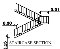
STAIRCASE SECTION
