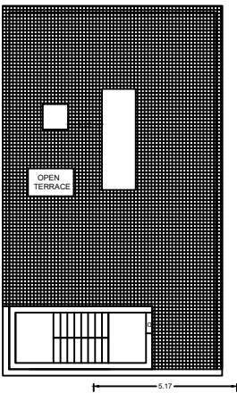
TERRACE FLOOR PLAN
