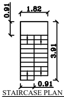
STAIRCASE PLAN
