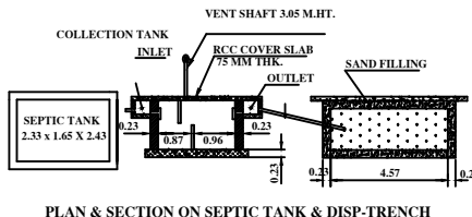
PLAN & SECTION ON SEPTIC TANK & DISP-TRENCH
