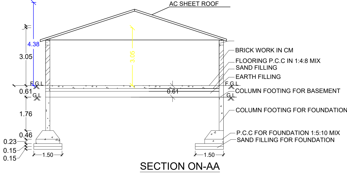
SECTION ON-AA
