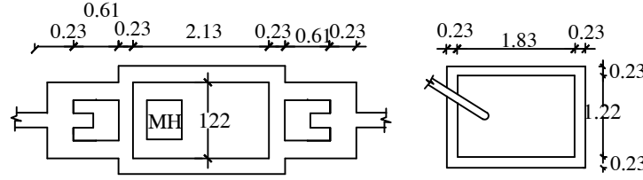
PLAN
