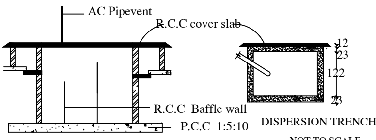
SEPTIC TANK
