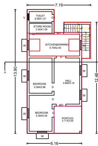
EXI.GROUND FLOOR PLAN
