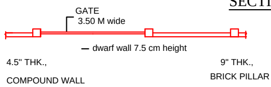
COMPOUND WALL PLAN
