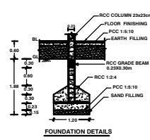
FOUNDATION DETAILS
