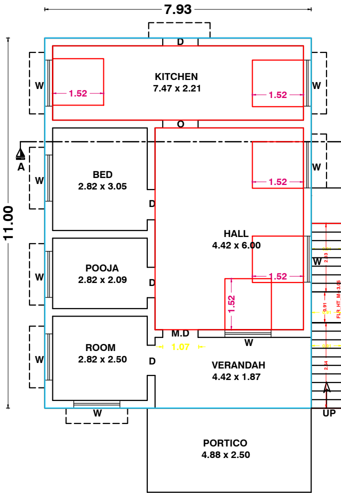
EXI.GROUND FLOOR PLAN
