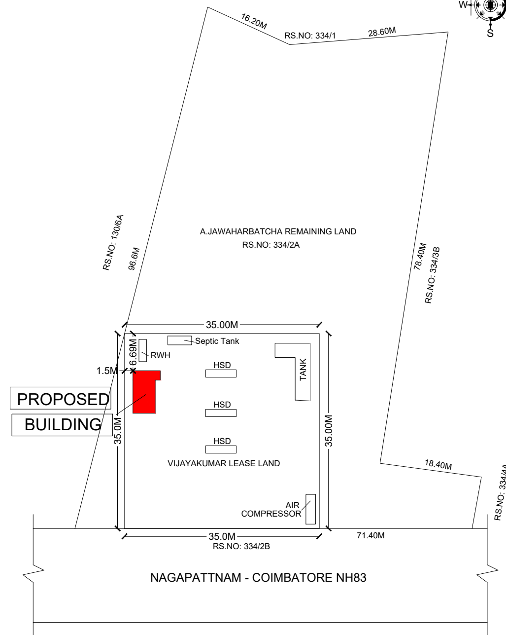
SITE PLAN
