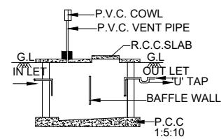
SEC. OF SEPTIC TANK
