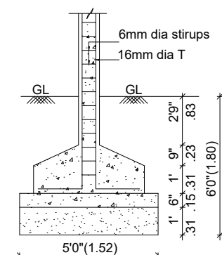
COLUMN FOUNDATION DETAIL SCALE (1:50)
