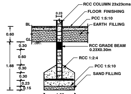
FOUNDATION DETAILS
