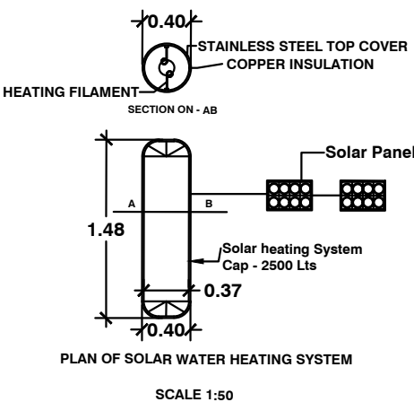
SCALE 1:50
