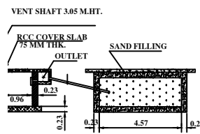
SEPTIC TANK & DISP-TRENCH
