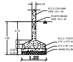
COLUMN FOUNDATION DETAILS
