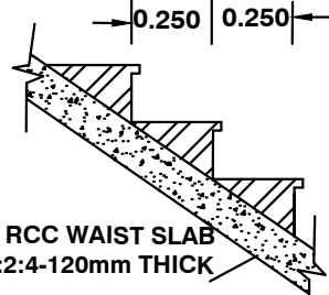
RCC WAIST SLAB 1:2:4-120mm THICK SCALE 1:25
