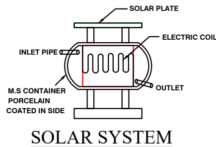
SOLAR SYSTEM
