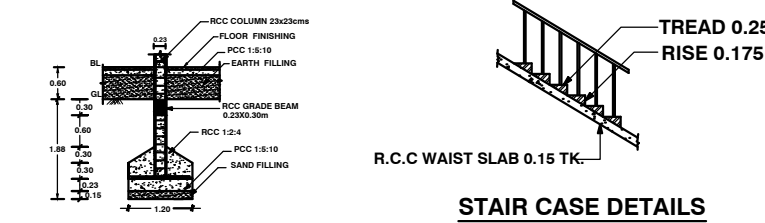
FOUNDATION DETAILS
