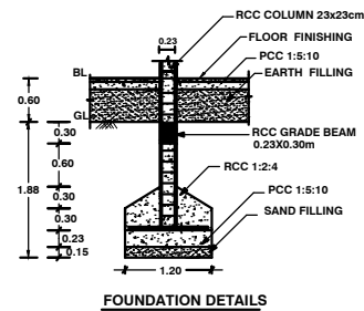
FOUNDATION DETAILS
