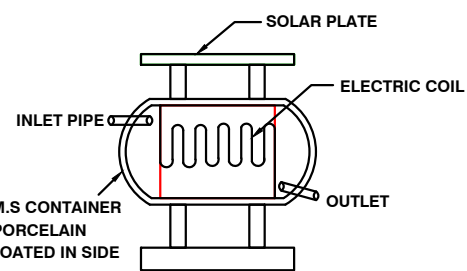
SOLAR SYSTEM
