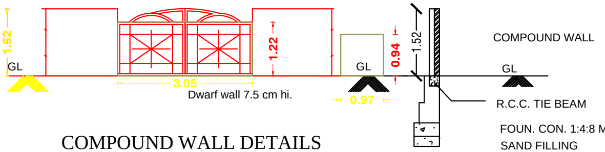
SECTION
