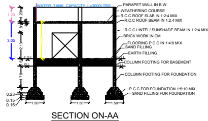
SECTION ON-AA
