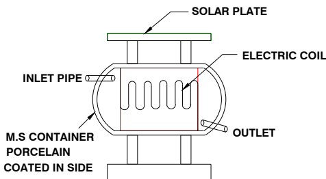
SOLAR SYSTEM
