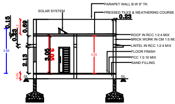
CROSS SECTION AB
