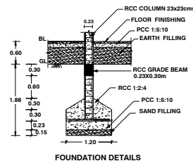
FOUNDATION DETAILS
