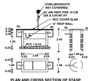
PLAN AND CROSS SECTION OF ST&P
