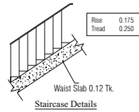
Staircase Details
