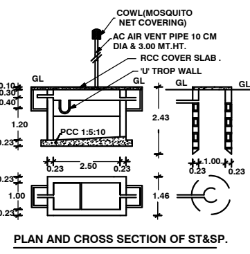
PLAN AND CROSS SECTION OF ST&SP.
