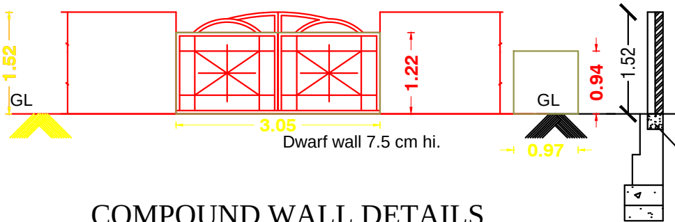
COMPOUND WALL DETAILS
