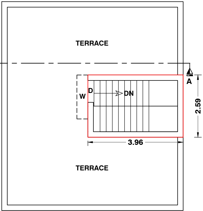
HEAD ROOM PLAN
