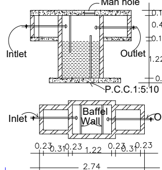
Plan & section of septic tank (Not to scale)
