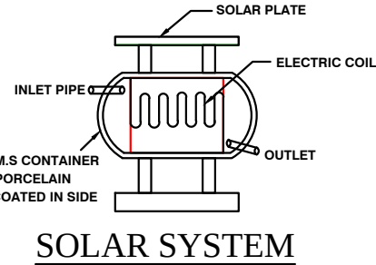
SOLAR SYSTEM
