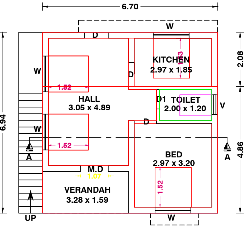
EXI & PRO.GROUND FLOOR PLAN
