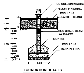
FOUNDATION DETAILS
