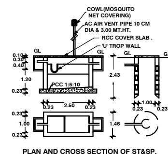
PLAN AND CROSS SECTION OF ST&amp;SP
