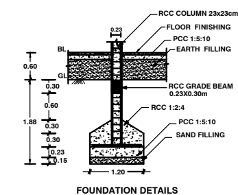
FOUNDATION DETAILS:
