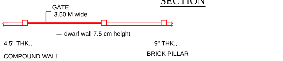
COMPOUND WALL PLAN
