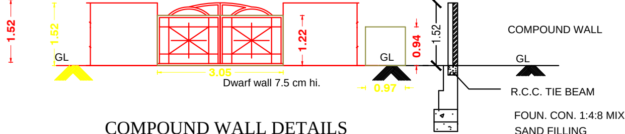
COMPOUND WALL DETAILS
