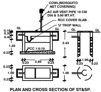
PLAN AND CROSS SECTION OF ST&SP.
