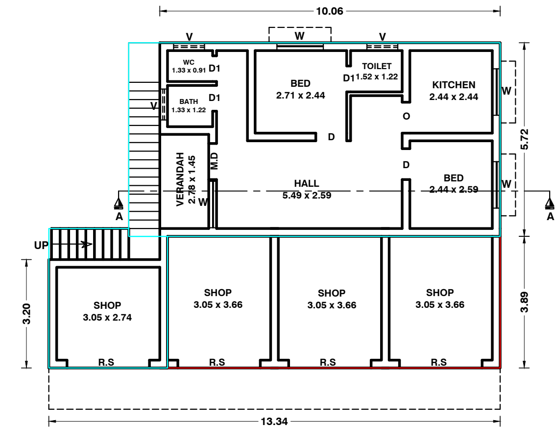
EXI. & PRO. GROUND FLOOR PLAN
