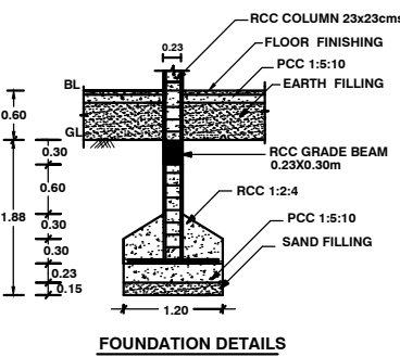
FOUNDATION DETAILS
