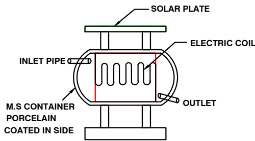
SOLAR SYSTEM
