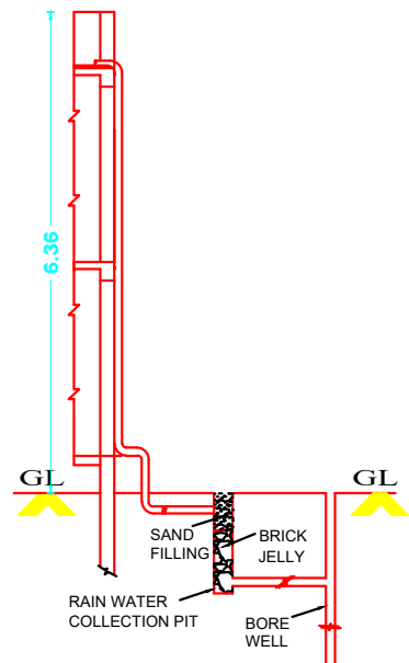
RAIN WATER HARVESTING SYSTEM RWH_CAPACITY_L=1000LTRS
