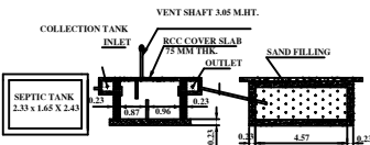
PLAN & SECTION ON SEPTIC TANK & DISP-TRENCH
