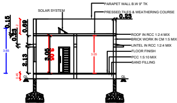
CROSS SECTION AB
