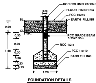
FOUNDATION DETAILS
