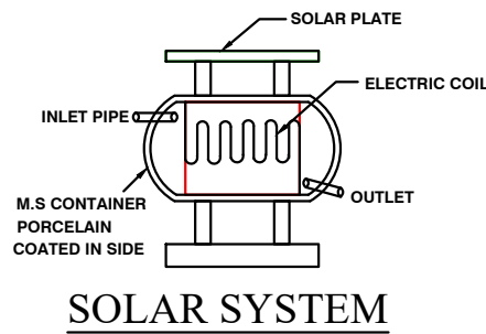
SOLAR SYSTEM
