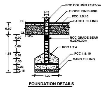
FOUNDATION DETAILS
