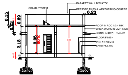
CROSS SECTION AB
