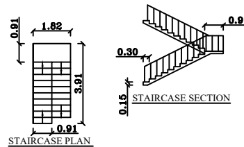
STAIRCASE PLAN
