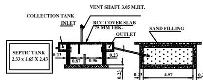
PLAN & SECTION ON SEPTIC TANK & DISP-TRENCH
