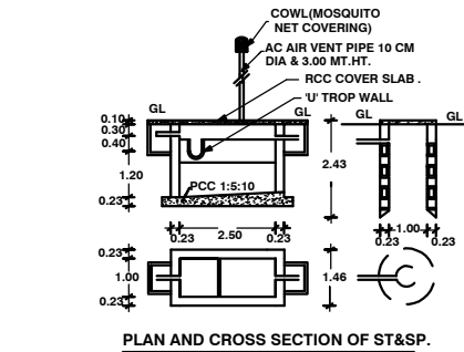
PLAN AND CROSS SECTION OF ST&SP.
