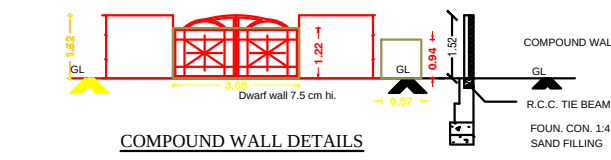
COMPOUND WALL DETAILS
