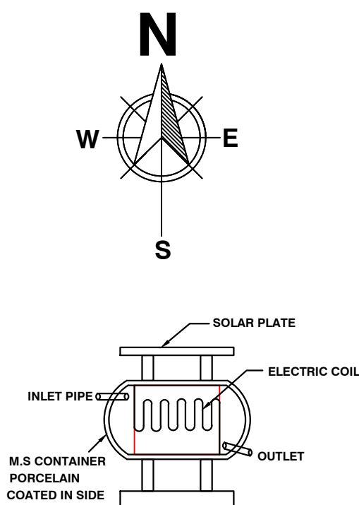
SOLAR SYSTEM
