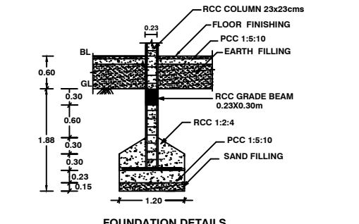
FOUNDATION DETAILS
