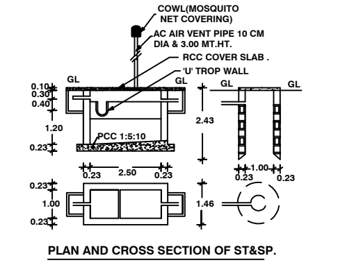
PLAN AND CROSS SECTION OF ST&SP.
