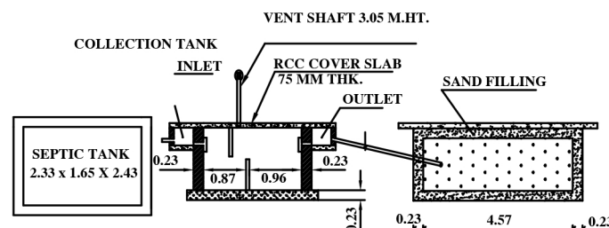
PLAN &amp; SECTION ON SEPTIC TANK &amp; DISP-TRENCH
