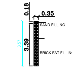
DETAILS OF PERCULATION PIT
