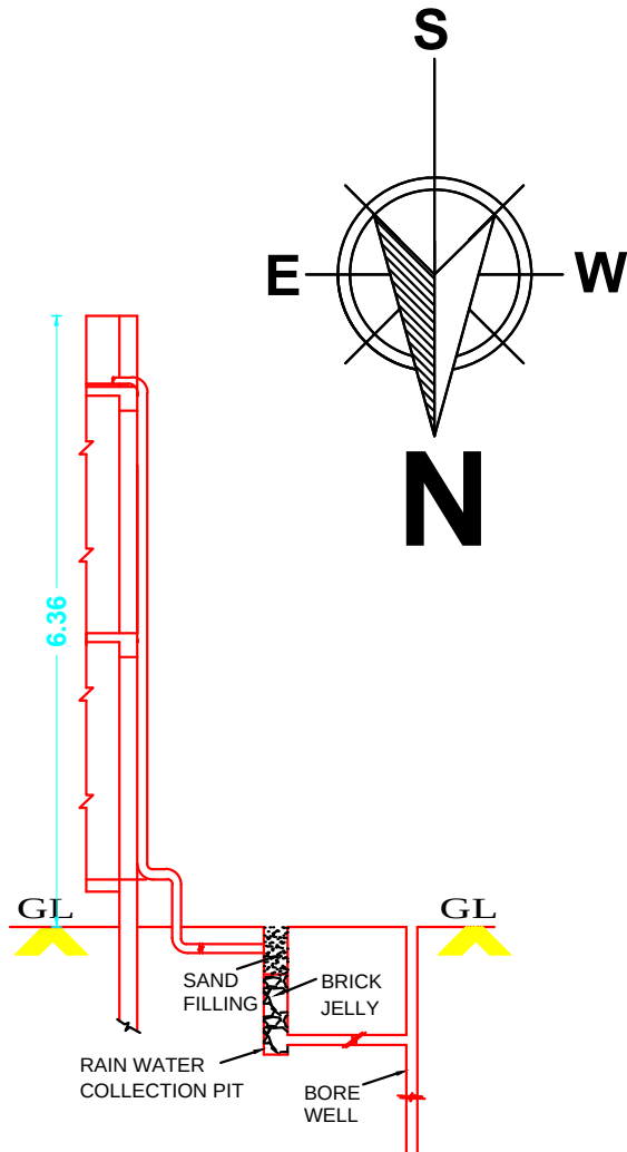
RAIN WATER HARVESTING SYSTEM RW_H_CAPACITY_L=1000LTRS
