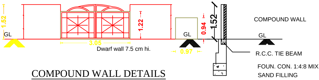
SECTION
