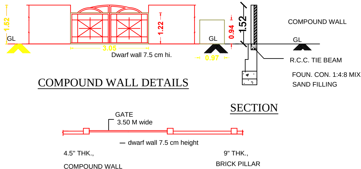
COMPOUND WALL PLAN
