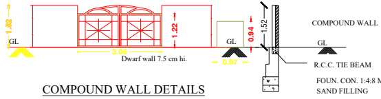
COMPOUND WALL DETAILS
