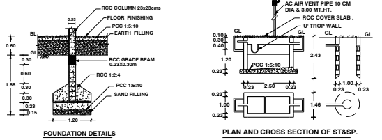
FOUNDATION DETAILS
